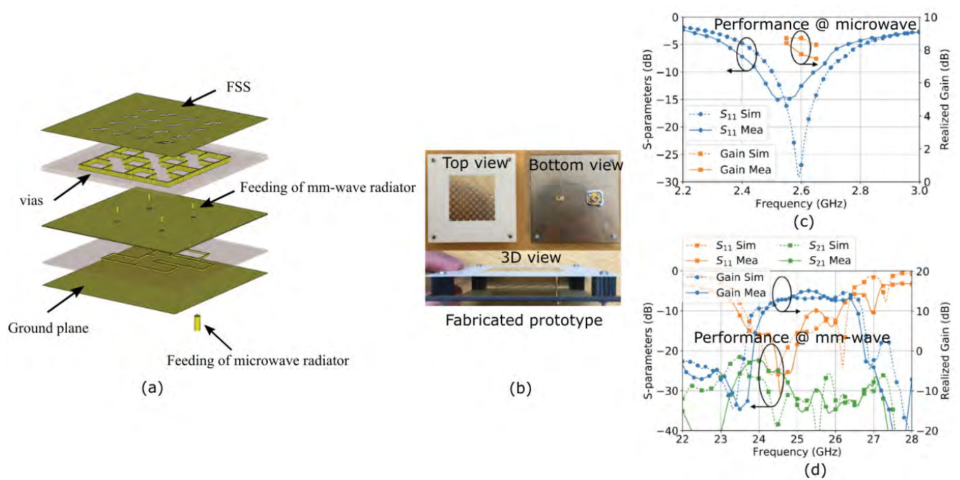
Figure 18. (a) Cavity-backed antenna integrated with FSS, (b) prototype of the antenna, (c,d) are simulated and measured S-parameters and gain at the lower and upper band [99].
