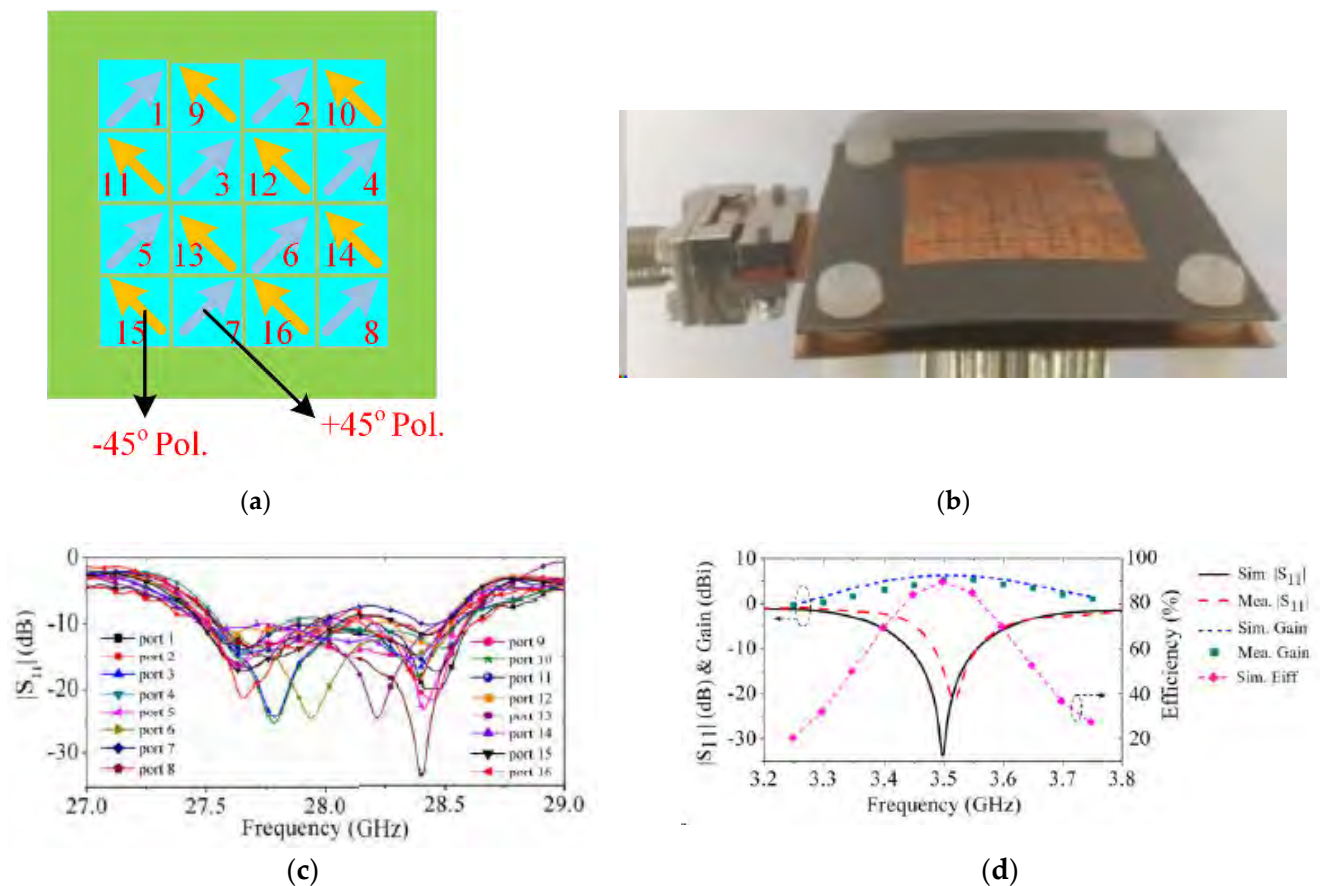
Figure 19. Configuration and results of the antenna from [97]: (a) antenna structure, (b) photo of the fabricated prototype (c) measured results at the mm-wave range, and (d) simulated and measured reflection coefficient and gain at the lower band.
