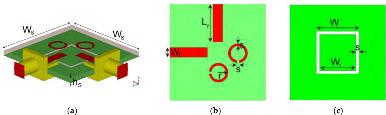
Figure 9. Dual-polarized square ring slot antenna [14]. (a) 3-D view, (b) Front view, (c) Back view.
