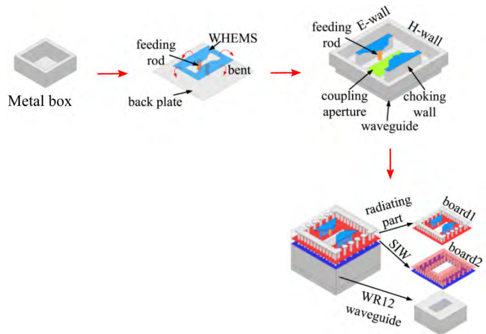
Figure 20. Design evolution of antenna in a package at 60 GHz presented in [107].
