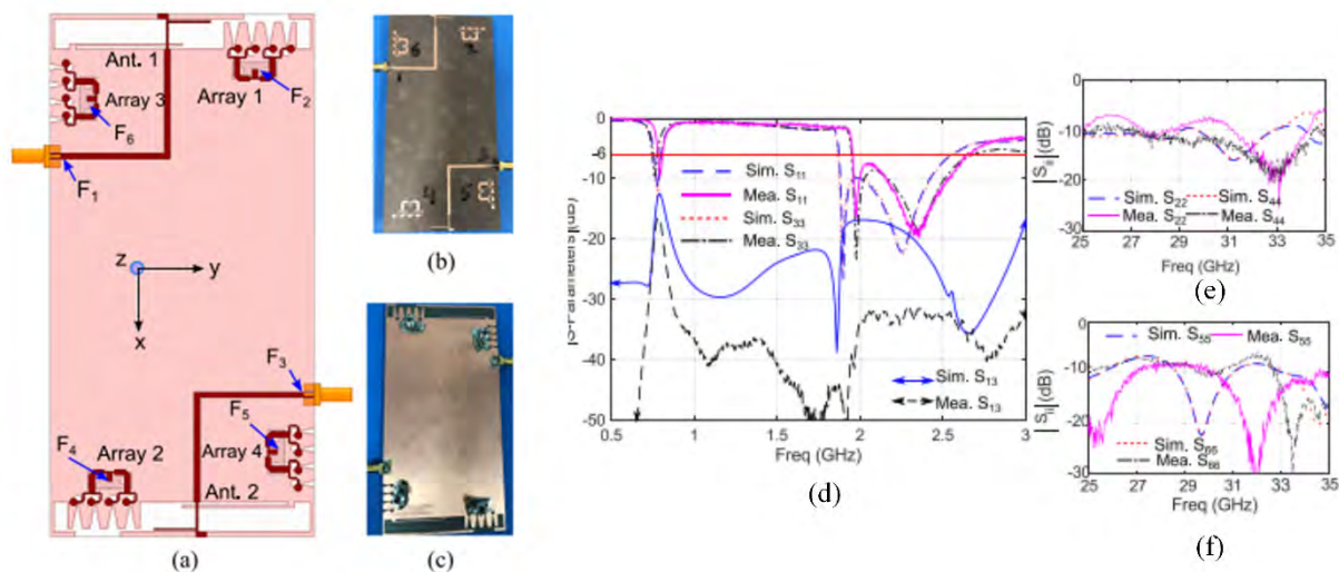
Figure 16. (a) Configuration of MIMO antenna, (b,c) are top and bottom views of the proposed antenna, and (d–f) simulated and measured S-parameters of the MIMO antenna [74].
