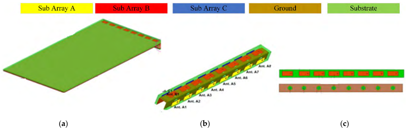
Figure 8. Switchable phased arrays (a) side view with full PCB, (b) 3 antenna arrays, and (c) top and bottom view of one array [13].
