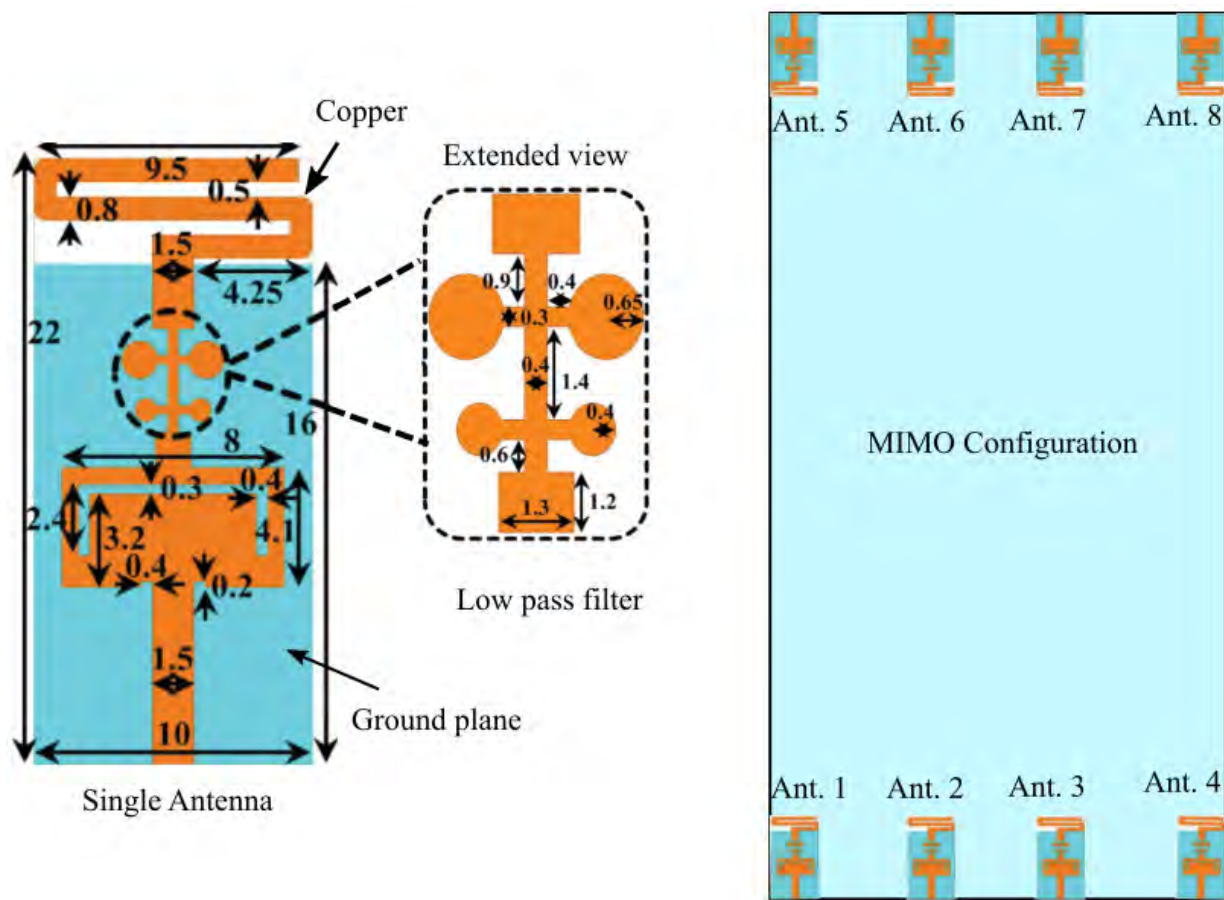
Figure 17. Structure of MIMO antenna that consists of 8 elements [98].
