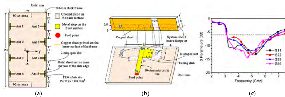
Figure 11. Eight–element MIMO antenna: [61] (a) configuration of the whole antenna, (b) detailed structure of slot antenna, and (c) measured reflection coefficient.
