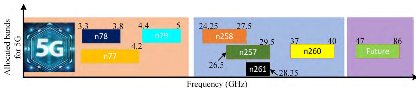
Figure 1. 5G allocated bands, the concept has been obtained from [20].
