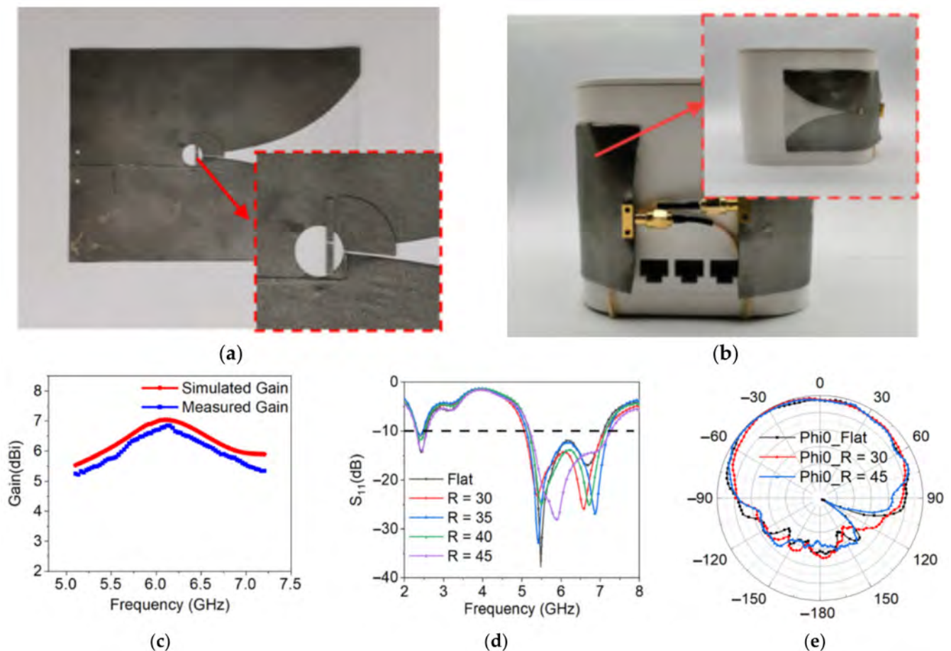
Figure 23. (a,b) Fabricated prototype and (c–e) some results of the conductive graphene-based conformal dual-band Vivaldi antenna [136].
