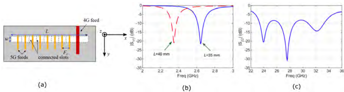
Figure 15. CSAA consists of 8 feeders for the mm-wave band and one feeder for the low band, (a) CSAA configuration, (b) reflection coefficient at lower band, and (c) reflection coefficient at the upper band.
