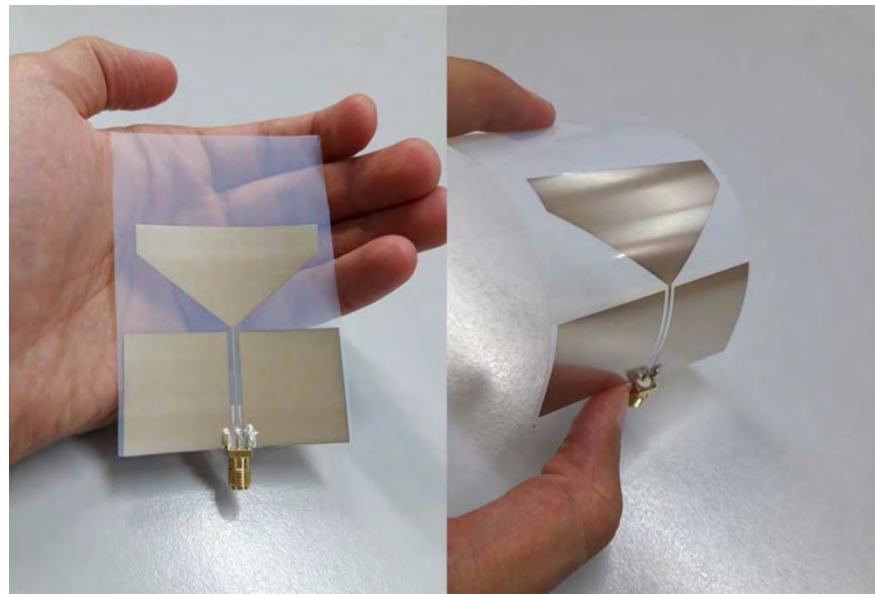
Figure 22. Fabricated prototype of the modified microstrip patch antenna (reused with permission) [132].
