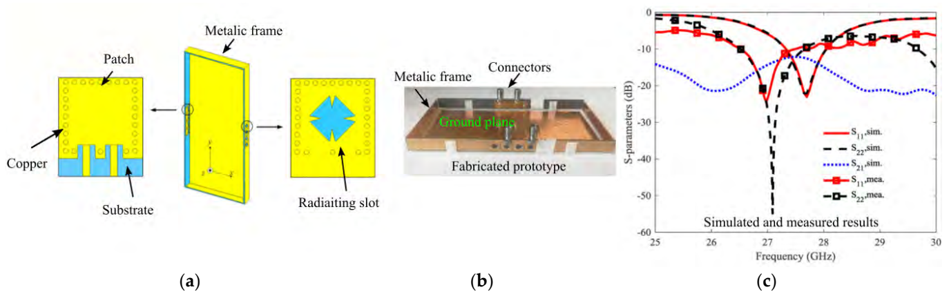
Figure 13. Dual-polarized frame integrated slot array [93] (a) configuration of the antenna array, (b) photo of the fabricated antenna, and (c) simulated and measured S-parameters.
