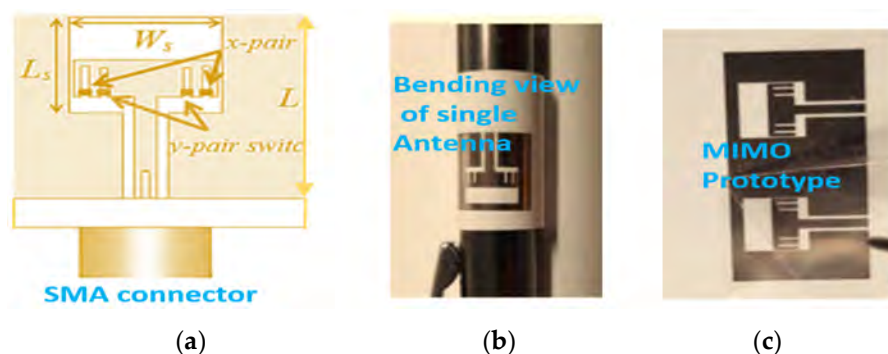
Figure 24. (a) The geometry and (b,c) prototype of the introduced mm-wave MIMO antenna in [142].
