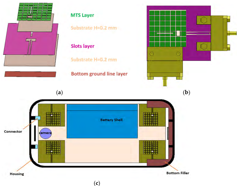
Figure 10. Configuration of the MIMO antenna with the MTS [30]; (a) 3D structure, (b) top view, and (c) view of the antenna inside mobile housing.
