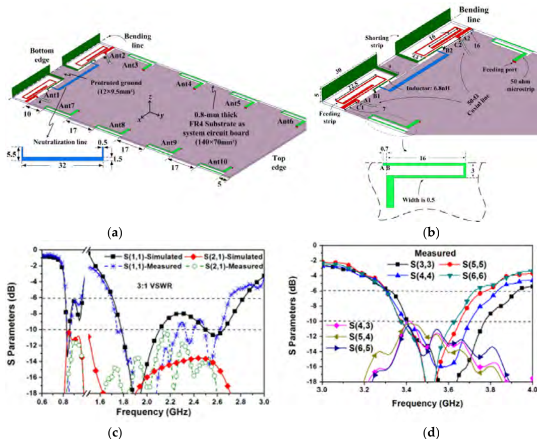
Figure 12. Configuration of MIMO antenna [69], (a) whole structure, (b) 4G and 5G modules, and (c,d) simulated and measured S–parameters.
