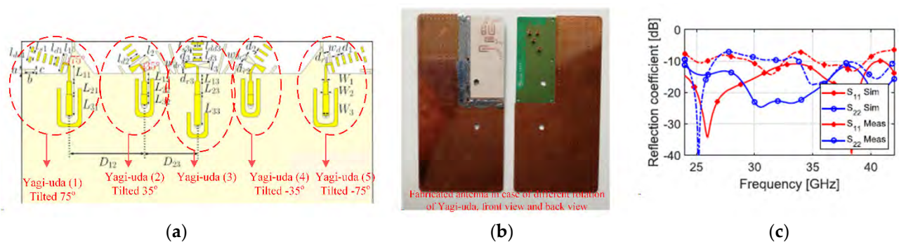
Figure 14. The proposed planar quasi-yagi-uda antenna in [65]: (a) geometry of the proposed antenna, (b) photo of the fabricated prototype, and (c) simulated and measured S-parameters.
