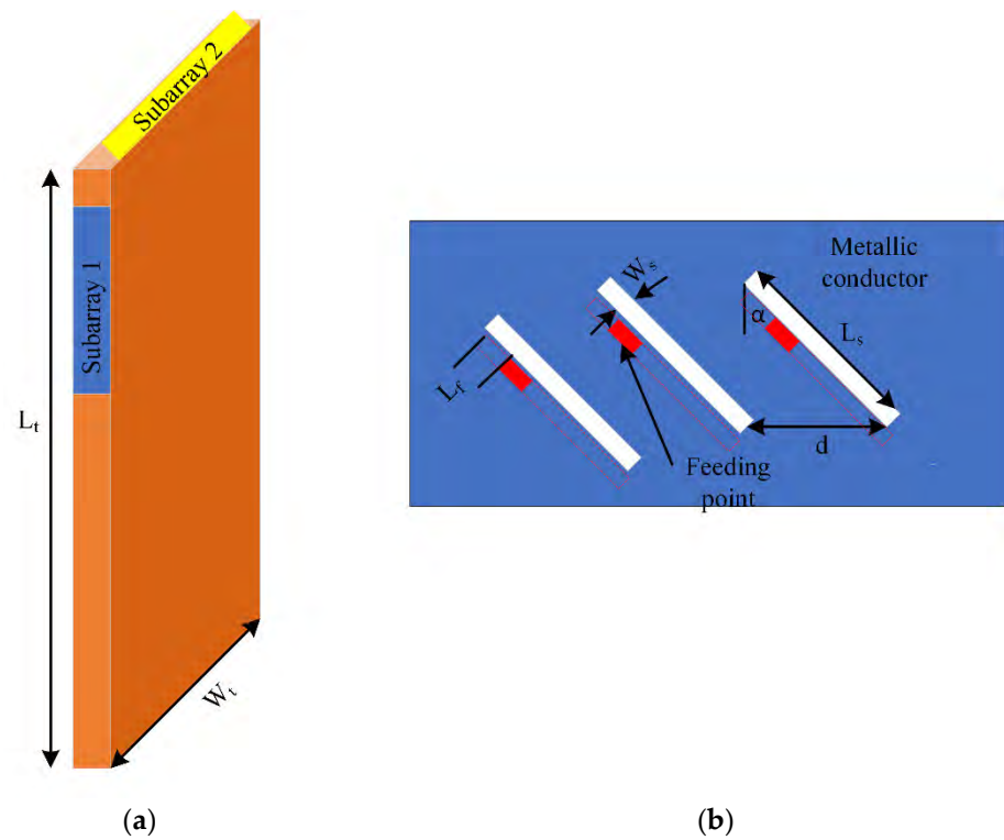
Figure 6. Steerable antenna array with full board (a) metallic frame view of the mobile handset (b) feeding details; the idea behind this figure brought from [7]. L_t = 67.1 , W_t = 17.28 , h_t = 7.1 , h_s = 1 , \alpha = 600 , L_s = 5.43 , d = 5.45 , W_s = 0.26 , L_f = 0.5 , L_g = 1 (units (mm)).
